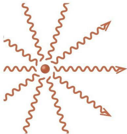
Rate of radioactive decay measured in becquerels or curies
